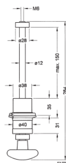
Feedthrough
